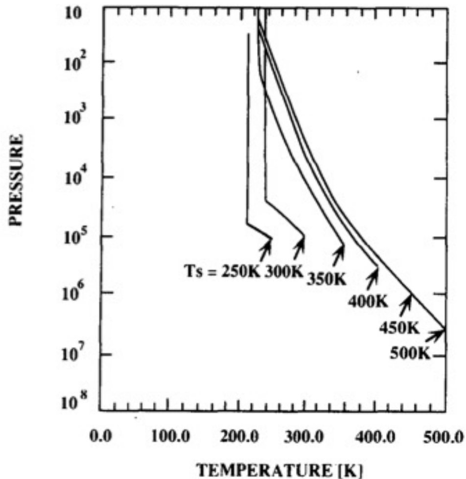
Atmospheric temperature
