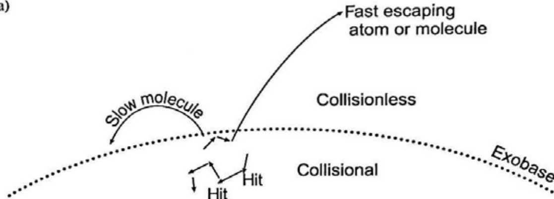
Figure 5.2 Schematic diagram of thermal escape end-members. (a) Jeans' escape is escape of molecules or atoms with an upward-directed component of velocity bigger than the escape velocity from the collisional part of the atmosphere into a virtually collisionless exosphere. (b) Transonic hydrodynamic escape is where the upper atmosphere has sufficient heating to produce a radial outward velocity u , at the speed of sound ( u_{\text{sound}} ) in the collisional part of the atmosphere at the radius labeled sonic level . Heating is typically by soft x-rays and extreme ultraviolet radiation (EUV). The atmosphere flows out to the vacuum of space driven by a pressure gradient (with the boundary condition set at the sonic level) and the supersonic flow reaches escape velocity, v_{\text{escape}} . At very high levels, the atmosphere will have very few collisions and the fluid assumption of hydrodynamic escape breaks down. However, under the transonic circumstances depicted, the fluid equations extrapolated to infinity provide a reasonable approximation to the density, temperature, and flow profiles.
