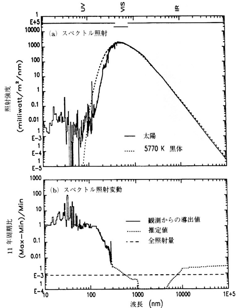
Solar spectrum
