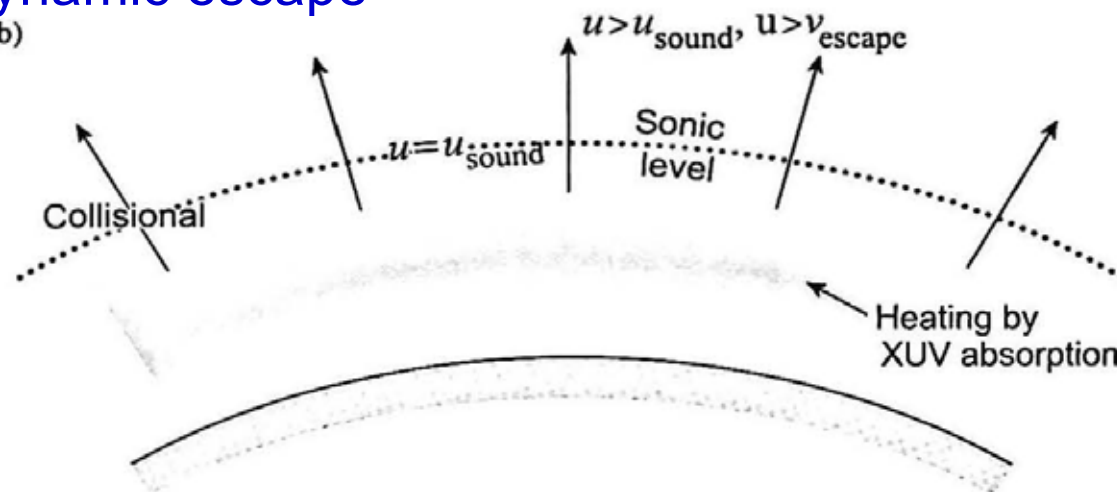
Figure 5.2 Schematic diagram of thermal escape end-members. (a) Jeans' escape is escape of molecules or atoms with an upward-directed component of velocity bigger than the escape velocity from the collisional part of the atmosphere into a virtually collisionless exosphere. (b) Transonic hydrodynamic escape is where the upper atmosphere has sufficient heating to produce a radial outward velocity u , at the speed of sound ( u_{\text{sound}} ) in the collisional part of the atmosphere at the radius labeled sonic level . Heating is typically by soft x-rays and extreme ultraviolet radiation (EUV). The atmosphere flows out to the vacuum of space driven by a pressure gradient (with the boundary condition set at the sonic level) and the supersonic flow reaches escape velocity, v_{\text{escape}} . At very high levels, the atmosphere will have very few collisions and the fluid assumption of hydrodynamic escape breaks down. However, under the transonic circumstances depicted, the fluid equations extrapolated to infinity provide a reasonable approximation to the density, temperature, and flow profiles.
