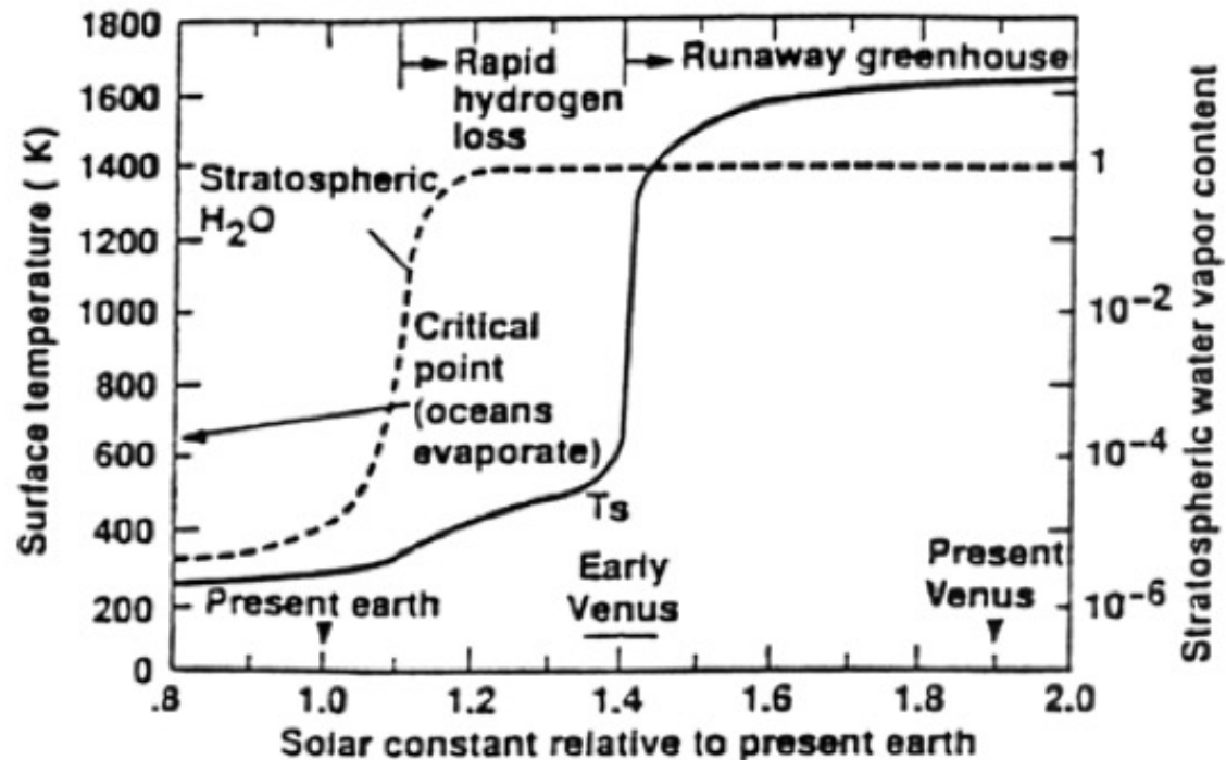
Fig. 1 Diagram illustrating what would happen to Earth if it were slowly pushed inwards towards the Sun. The horizontal scale is the solar flux relative to its value at 1 AU. The solid curve represents mean global surface temperature ( left-hand scale ). The dashed curve represents stratospheric H 2 O mixing ratio ( right-hand scale ). The solar flux at Venus today and at 4.5 billion years ago is indicated (adapted from Kasting 1988)
