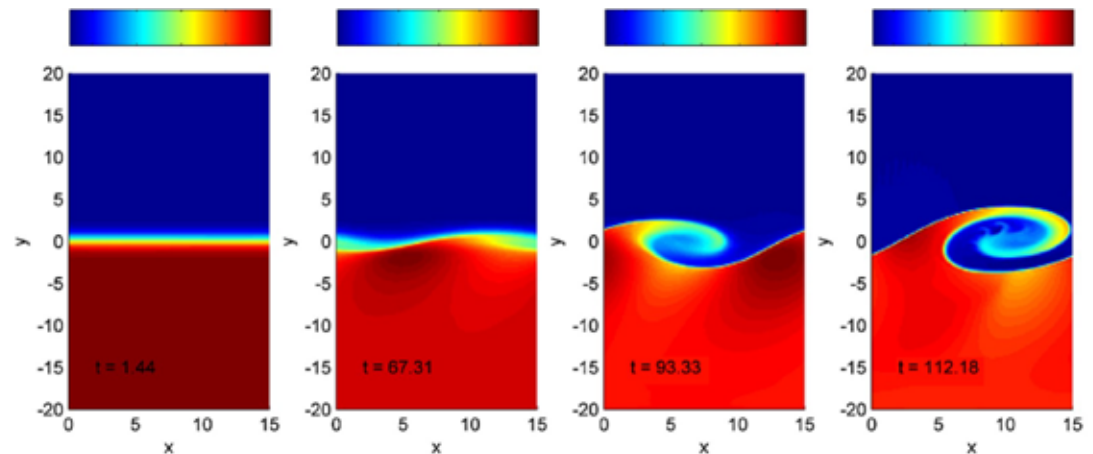
Fig. 12 Nonlinear evolution of the Kelvin-Helmholtz instability. The time series of the mass density is shown, from an MHD simulation with periodic boundary conditions in the x -direction. The mass density changes from the upper to the lower plasma layer and exhibits an increase of up to ten times (see the color code; blue : low density, red : high density). In the upper layer, the plasma flows from left to right . In the lower layer, the plasma is at rest. Initially small perturbations of the boundary layer separating the two plasma layers
