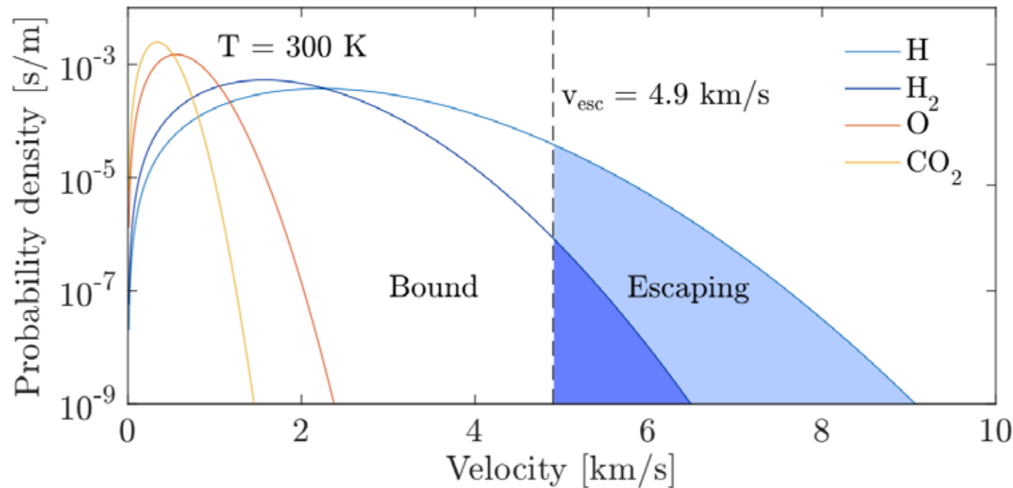
Figure 1.7: Thermal velocity distributions for several species in an example 300 K gas as described by the Maxwellian function (eq. 1.8). Only the H and H 2 distributions exhibit significant fractions above escape velocity near the exobase (4.9 km/s, marked by dashed line), in this case 0.023 % for H 2 and 2.1% for H. However, the Maxwellian distribution is isotropic, thus half these percentages will return to the atmosphere.
