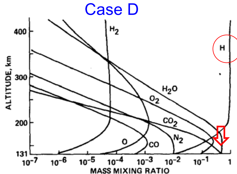
FIG. 10. Mass mixing ratio profiles for Case D.
