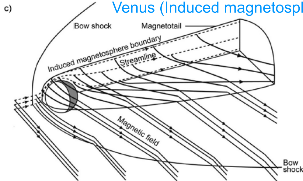
Fig. 5 Comparison of three different magnetospheres. The Earth's magnetosphere (a) is a typical example of an intrinsic magnetosphere. Venus magnetosphere is overlaid as a dashed line to illustrate the difference in size (adopted from Luhmann 1991a). A cometary induced magnetosphere is characterized by the draping of the solar wind magnetic field (b) introduced by the mass loading process (adopted from Russell et al. 2016). The induced magnetosphere of Venus (c) is a typical example of a magnetosphere of unmagnetized atmospheric object (adopted from Saunders and Russell 1986). Solar wind interaction to Mars exhibits similar interaction to Venus
