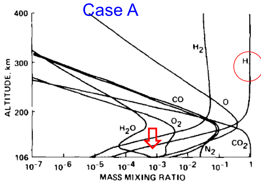
FIG. 9. Mass mixing ratio profiles for Case A.
